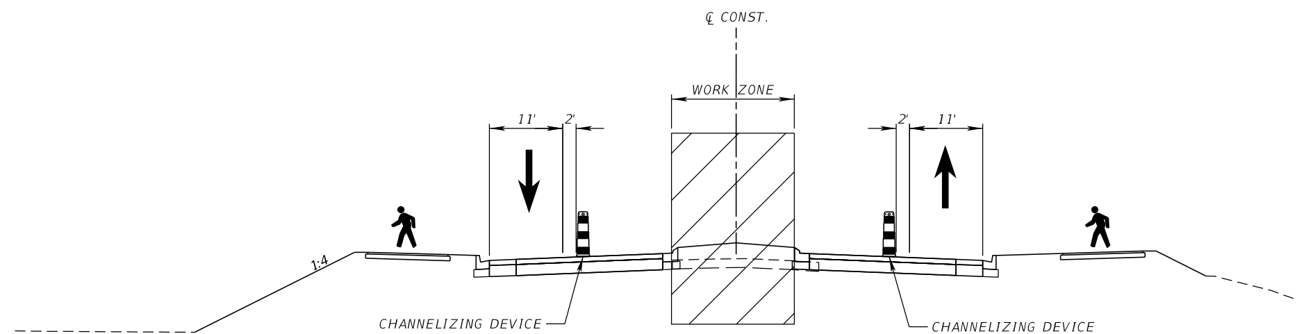
PHASE 4 STA. 2+00 TO END PROJECT
