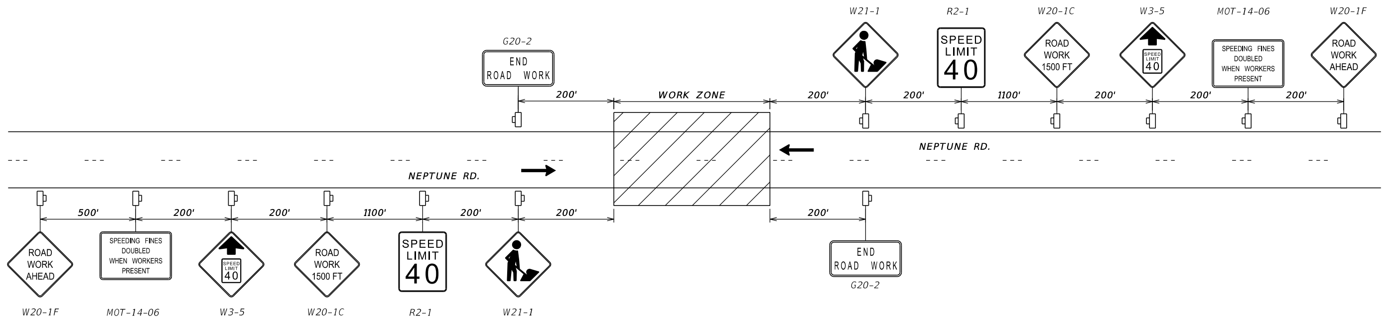
NEPTUNE ROAD ADVANCED WARNING SIGNS DETAIL N.T.S.
