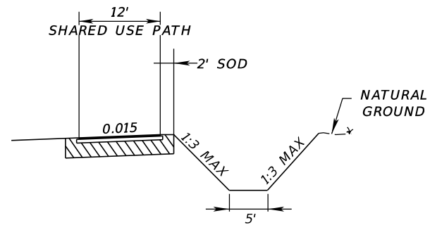
OUTFALL DITCH DETAIL
