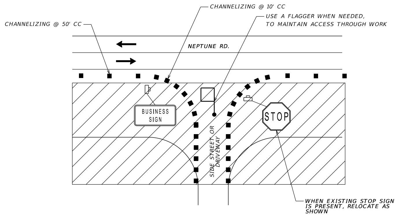
SIDE STREET AND DRIVEWAY ACCESS THROUGH WORK ZONE DETAIL N.T.S.
