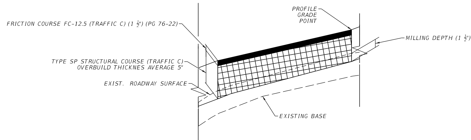
NEPTUNE ROAD MAINLINE OVERBUILD AND RESURFACING DETAIL
