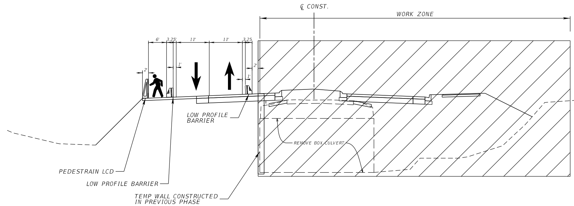
PHASE 3 STEP 3 EXIST. FISH LAKE BOX CULVERT
