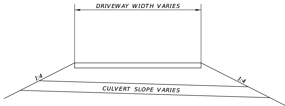
DRIVEWAY CULVERT SECTION DETAILS
