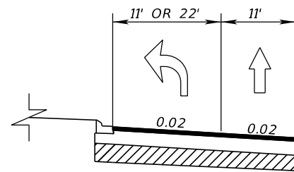
LEFT TURN LANE DETAIL
