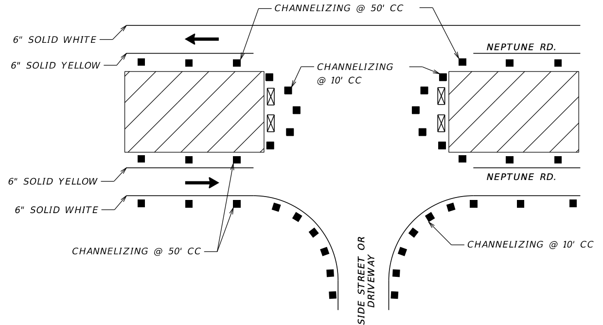
MEDIAN OPENING CHANNELIZING SPACING AND PAVEMENT MARKINGS DETAIL N.T.S.
