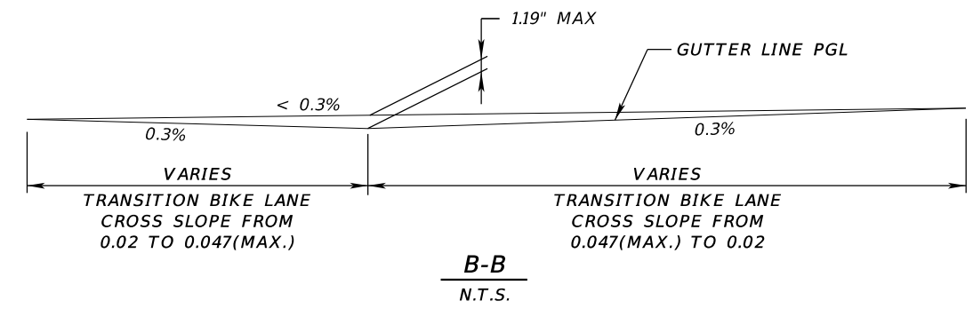
BIKE LANE ROCKING DETAIL WHEN PGL < 0.3%
