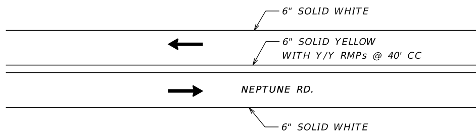
PAVEMENT MARKINGS 2-WAY UNDIVIDED SECTION DETAIL N.T.S.
