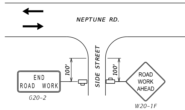
SIDE STREET ADVANCED WARNING SIGNS DETAIL N.T.S.
