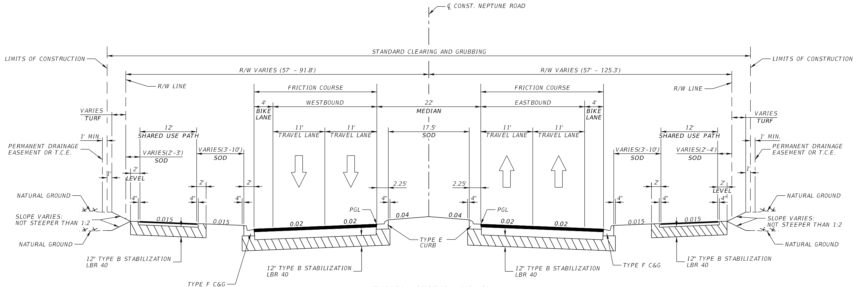
TYPICAL SECTION NO. 2 NEPTUNE ROAD STA. 6+00.00 TO STA. 28+00.00 (WB) STA. 7+50.00 TO STA. 28+00.00 (EB) STA. 30+50.00 TO STA. 74+92.75 (WB & EB)
