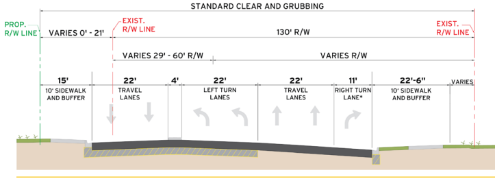
TYPICAL SECTION | SIMPSON ROAD
