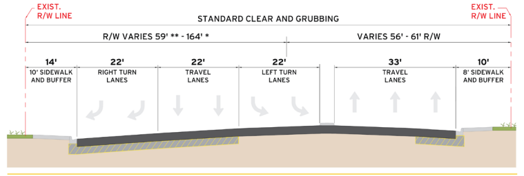
TYPICAL SECTION | SIMPSON ROAD
