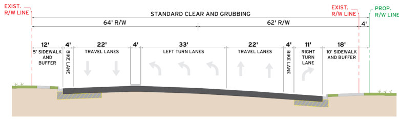
TYPICAL SECTION | FORTUNE ROAD
